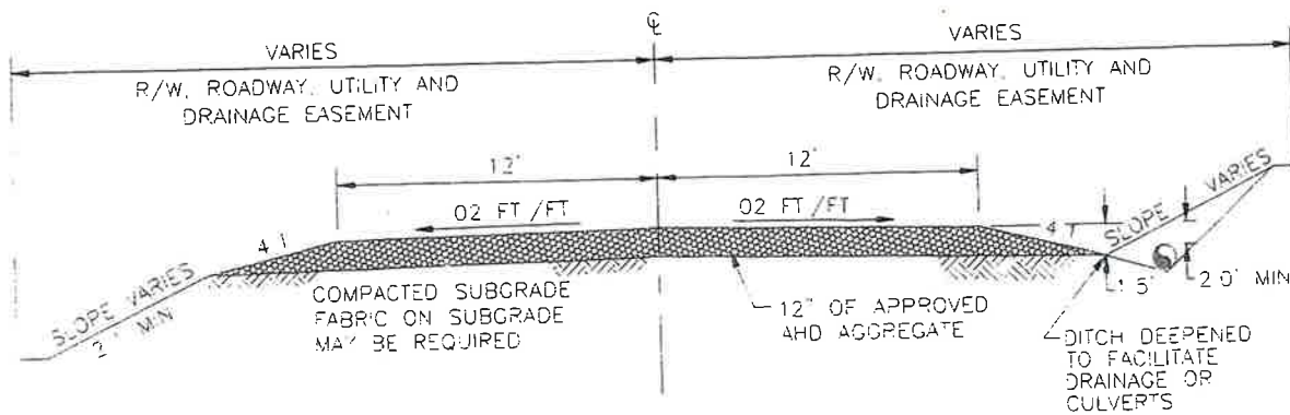
SUPPLEMENTAL SD-1B PRIVATELY MAINTAINED GRAVEL ROAD SECTION N T S
